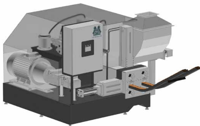
The BPH Quattro Hydraulic Briquetting Press with consumer briquettes.
